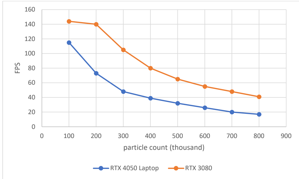
9. Figure: FPS as a function of particle count
